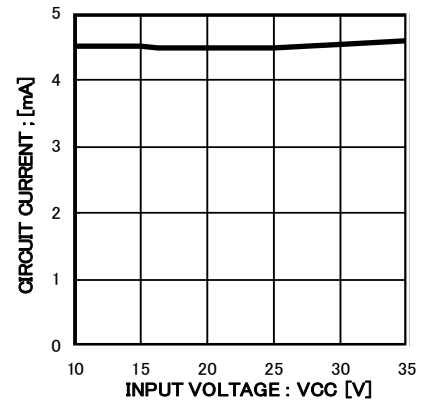
Fig.24 CIRCUIT CURRENT-INPUT VOLTAGE NO LOAD
