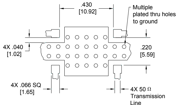
Dimensions are in Inches [Millimeters] XC1900A-20* Mounting Footprint
