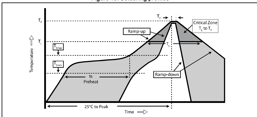
Figure 15: Soldering profiles
