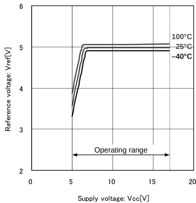
Fig.18 Reference voltage
