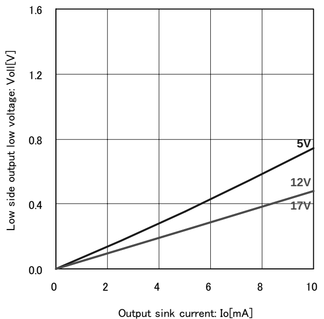
Fig.10 Low side output low voltage ( T_a=25^{\circ}C )
