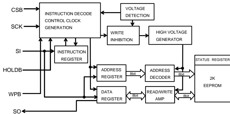
Figure 5. Block diagram
