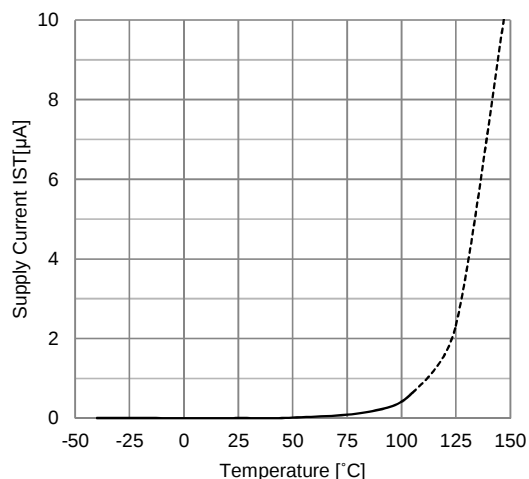
Supply Current vs. Temperature [Standby] V^+ = +3.3V , R_L = \text{Open} , V_{\text{pullup}} = +3.3V , No signal
