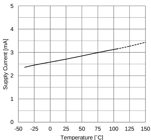
Supply Current vs. Temperature V^+ = +3.3V , R_L = \text{Open} , No signal
