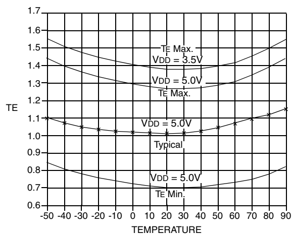
FIGURE 9-7: HCS320 TE VS. TEMP (BY CHARACTERIZATION ONLY)
