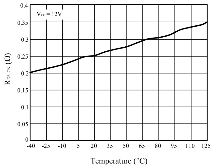
Figure 8 R_{DS\_ON} vs. Temperature
