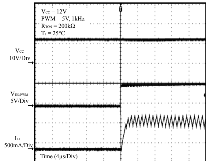
Figure 24 PWM On
