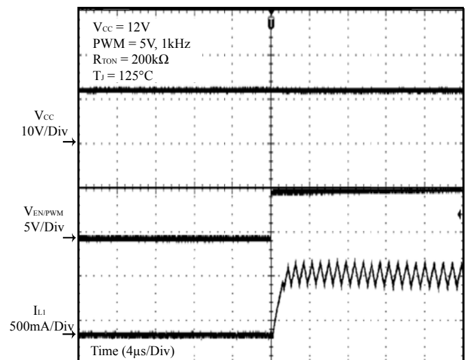
Figure 26 PWM On
