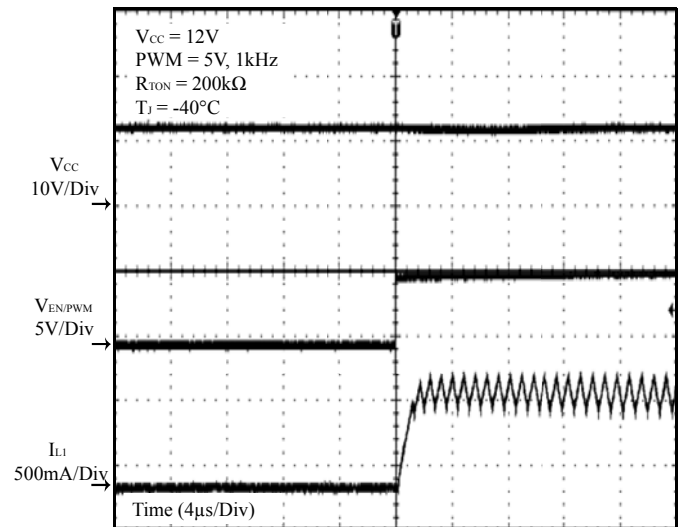
Figure 22 PWM On
