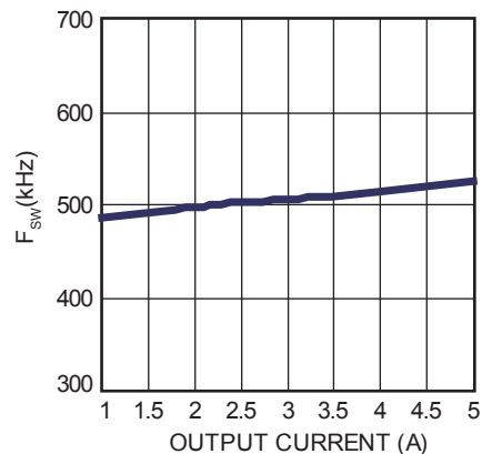
F_{SW} vs. Output Current
