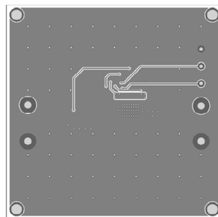
Figure 4—Inner2 Layer
