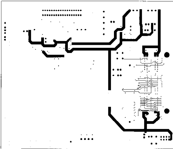
Figure 26. Power Plane 2
