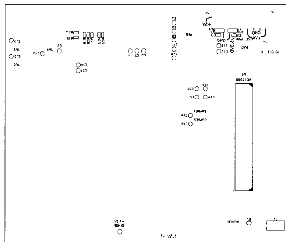
Figure 33. Bottom Silkscreen
