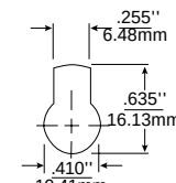
Keyhole Punch
