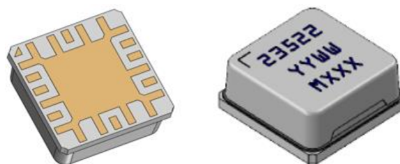
QFN 4x4 mm 22L
