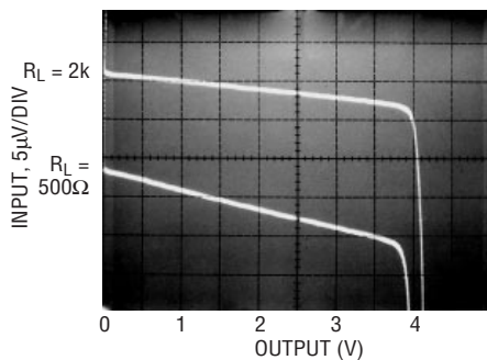
Open-Loop Gain, V_S = 5V
