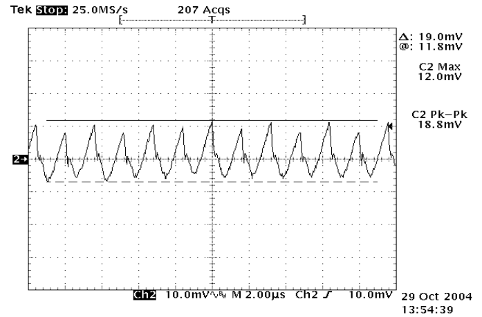
Figure 14: Output ripple & noise at 12Vin, 5V/40A out
