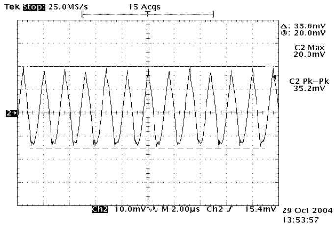
Figure 13: Output ripple & noise at 12Vin, 3.3V/40A out
