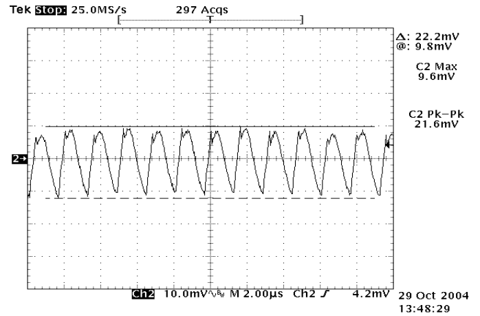
Figure 8: Output ripple & noise at 12Vin, 0.9V/40A out
