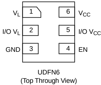
Figure 2. Pinout Diagram
