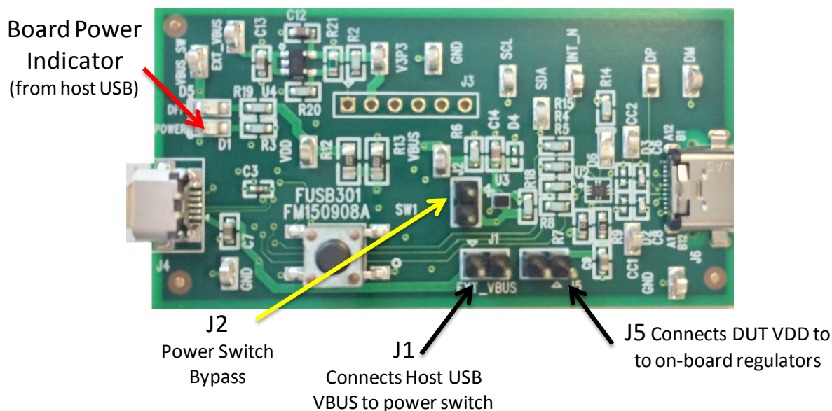
Figure 3 - FUSB301 Evaluation Board Power Configuration
