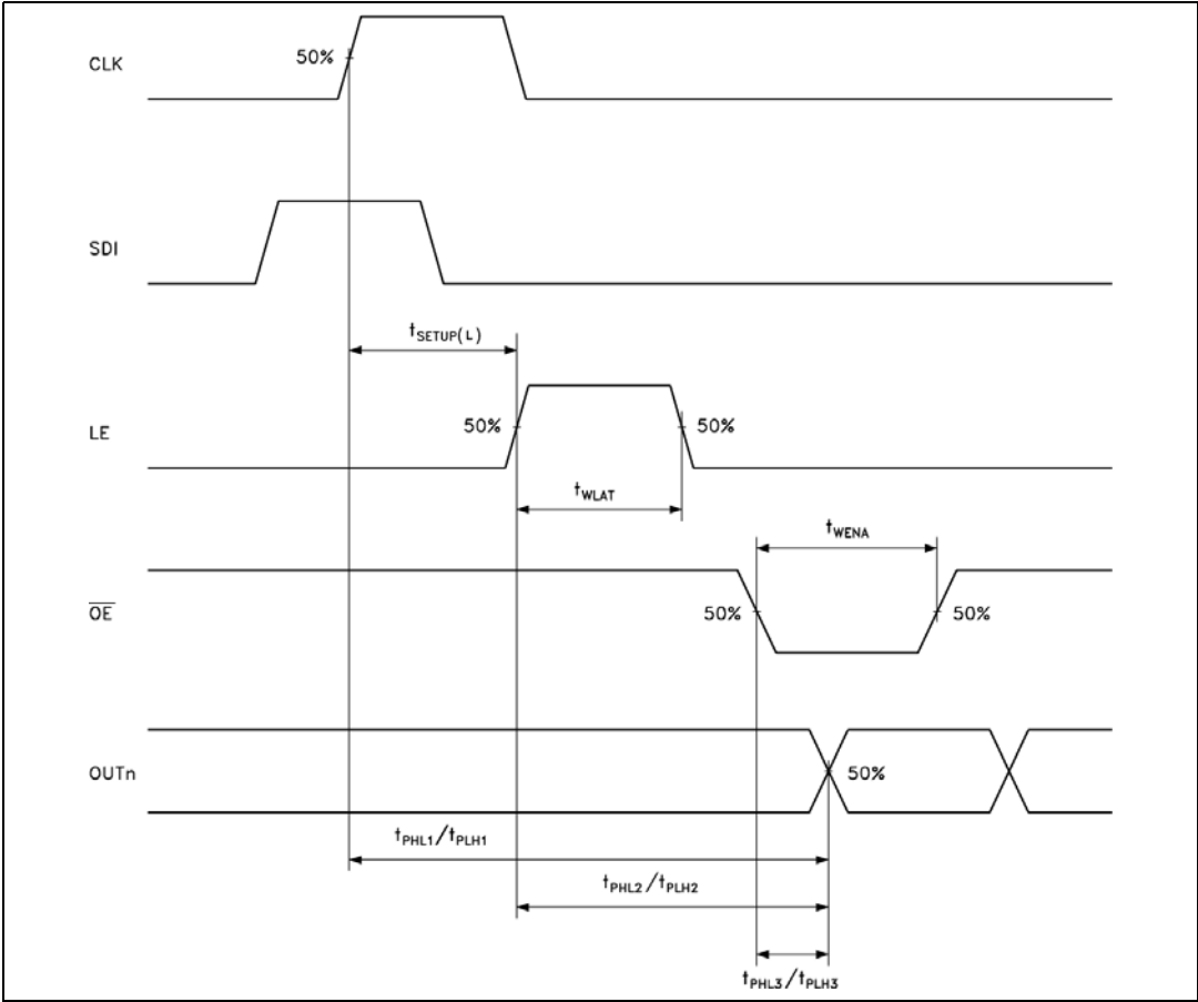
Figure 9. Clock, serial-in, latch, enable, outputs
