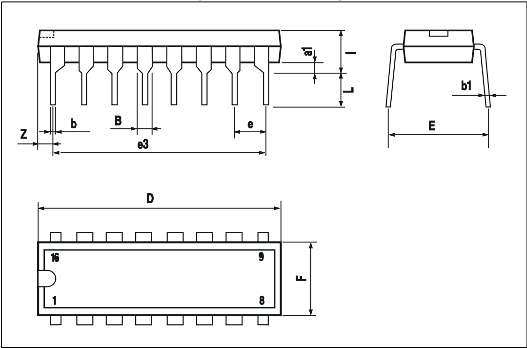
Figure 17. DIP-16 drawing
