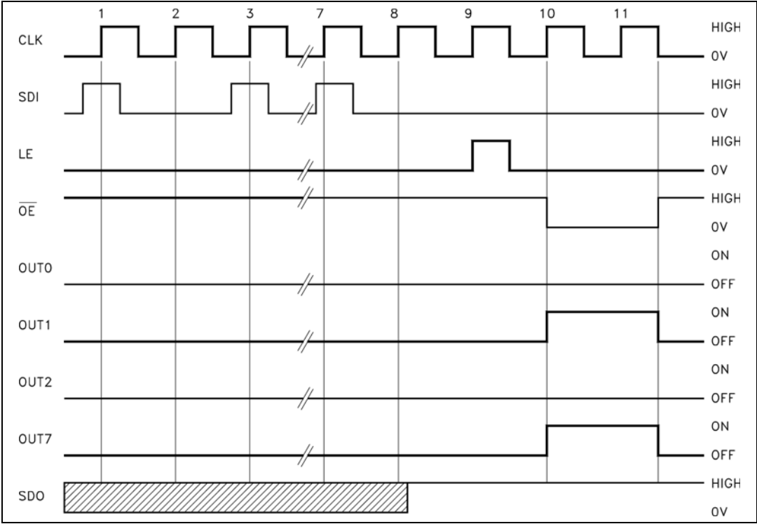
Figure 7. Timing diagram
