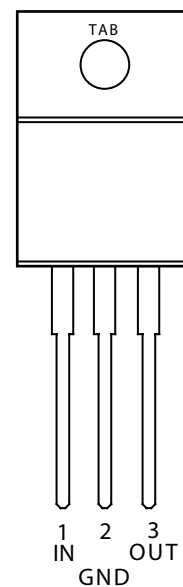
MIC2920A-xxBT (TO-220)
