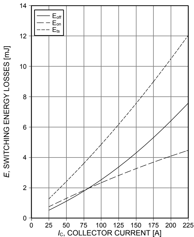
Figure 11. Typical switching energy losses as a function of collector current (inductive load, T_{vj}=150^{\circ}C , V_{CE}=400V , V_{GE}=0/15V , R_{Gon}=22,3\Omega , R_{Goff}=22,3\Omega , dynamic test circuit in Figure E)
