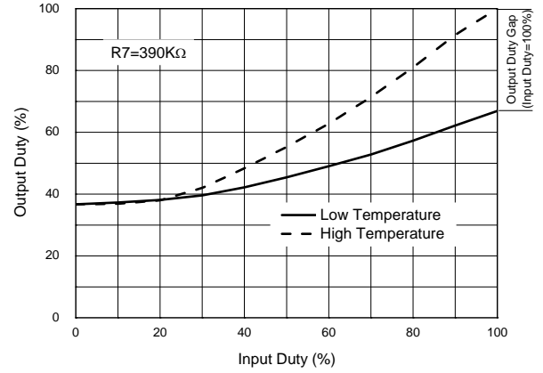
Output PWM Duty vs. Input PWM Duty with R7 (390kΩ)
