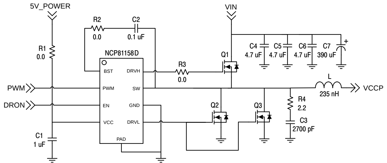
Figure 2. Application Circuit
