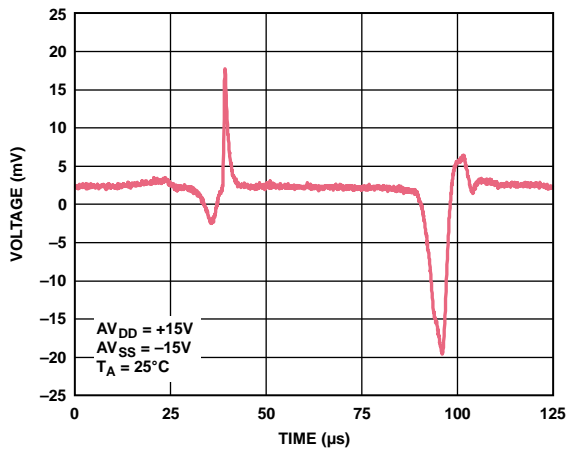
Figure 28. Voltage vs. Time on Power-Up
