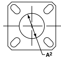
VIEW D FOR SIZE 8 TWINAX ONLY, RELATIVE TO -A-
