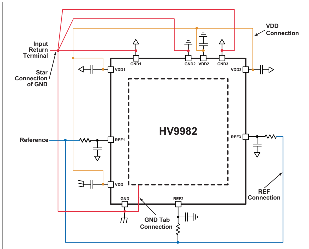
FIGURE 3-2: LAYOUT GUIDELINES
