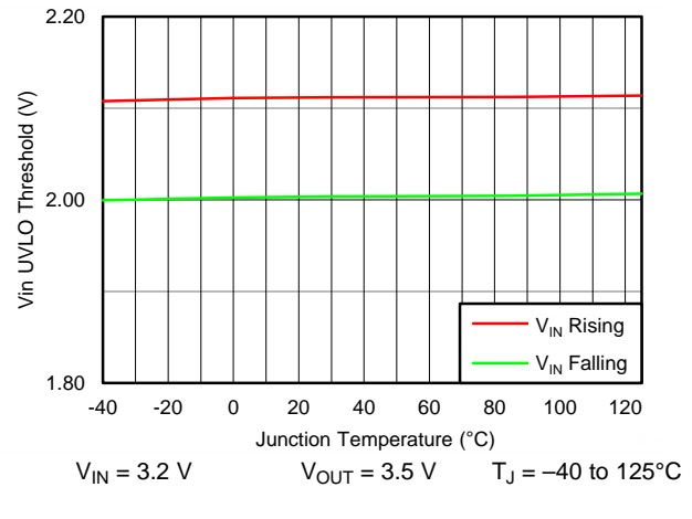
Figure 12. VIN UVLO Threshold Rising/Falling vs Junction Temperature
