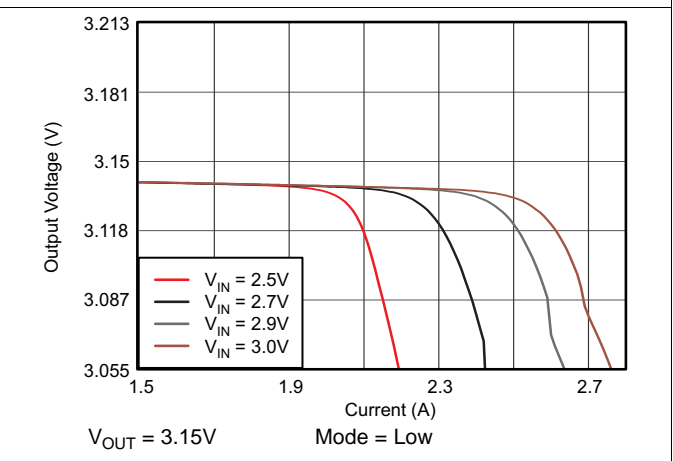
Figure 34. TPS61281 DC Output Voltage vs Output Current
