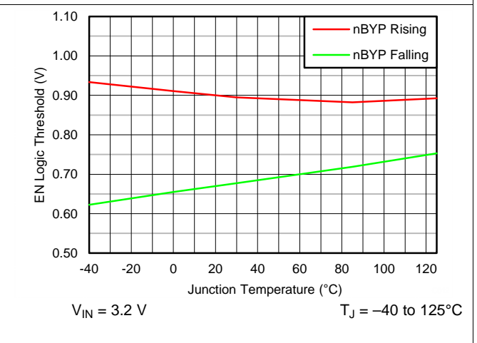
Figure 14. \overline{\text{BYP}} Logic High Threshold Rising/Falling vs Junction Temperature
