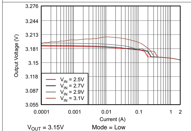
Figure 33. TPS61281 DC Output Voltage vs Output Current
