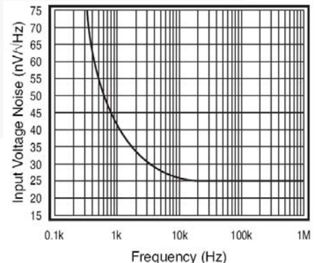
Figure 19. Input Voltage Noise
