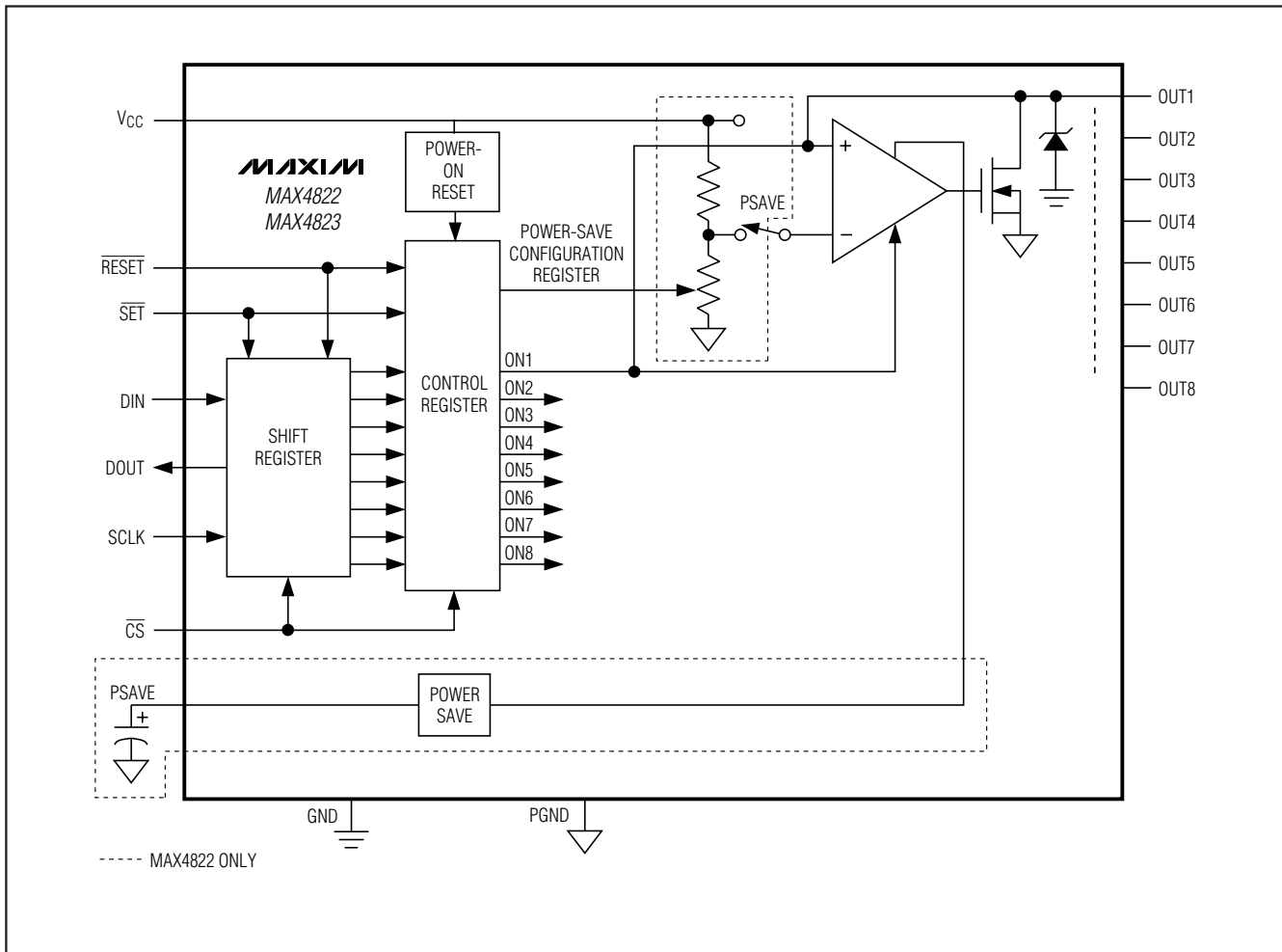
MAX4822/MAX4823 Functional Diagram (Serial Interface)
