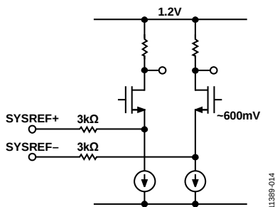
Figure 50. \text{SYSREF}_{\pm} Input Circuit
