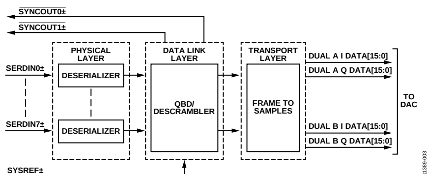
Figure 41. Functional Block Diagram of Serial Link Receiver
