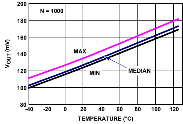
FIGURE 32. EL8173 V_{OUT} LOW vs TEMPERATURE, R_L = 1k , V_+ = \pm 2.5V
