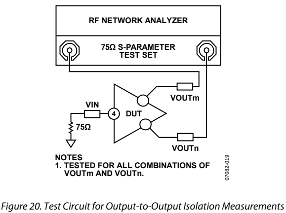
Figure 20. Test Circuit for Output-to-Output Isolation Measurements
