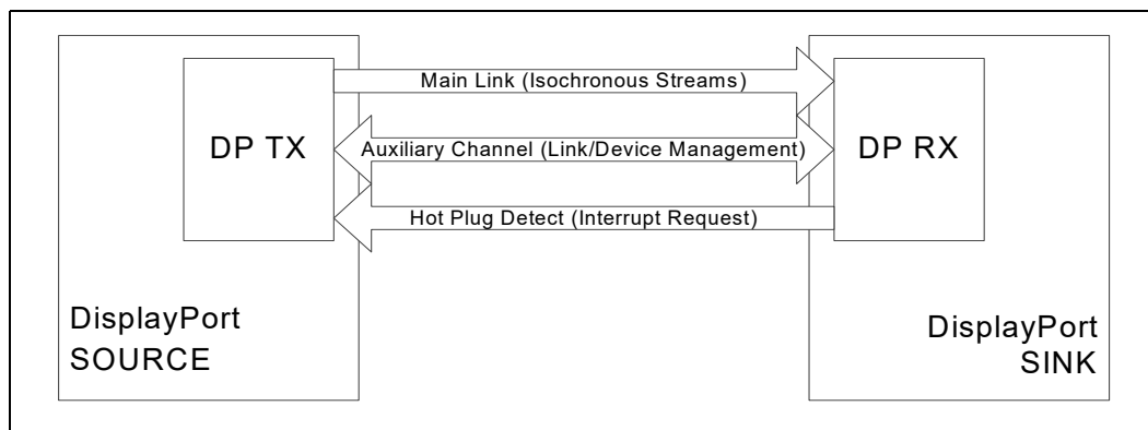
Figure 92. DisplayPort* Overview
