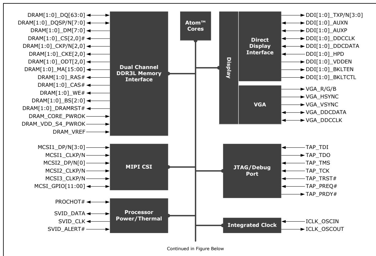
Figure 2. Signals (1 of 2)
