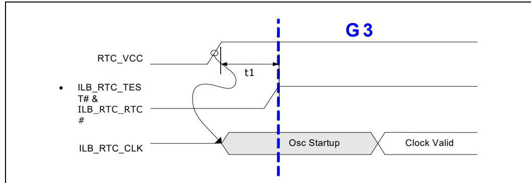
Figure 11. RTC Power Well Timing Diagrams
