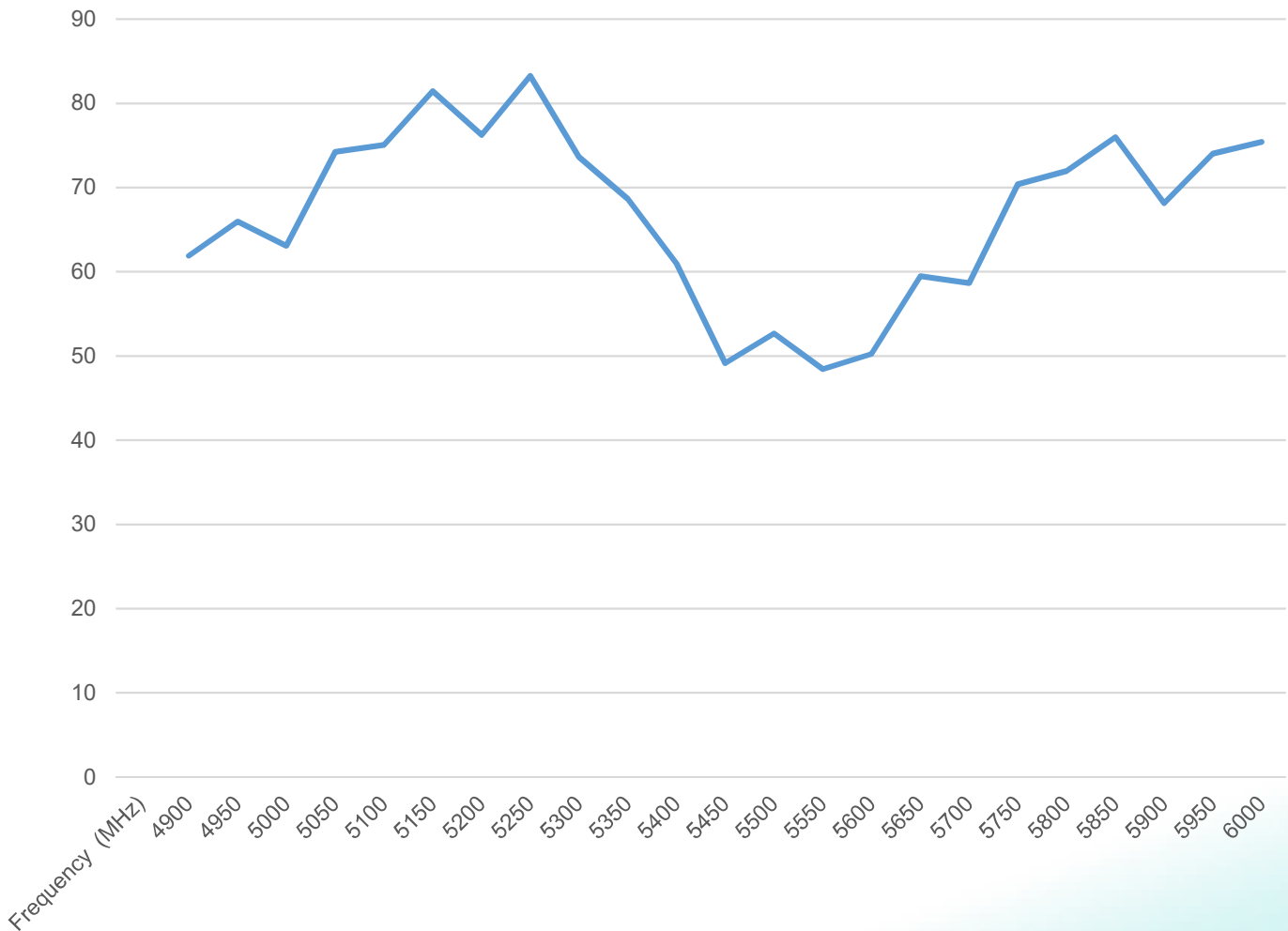
ICEFIN49DMN Efficiency (%)
