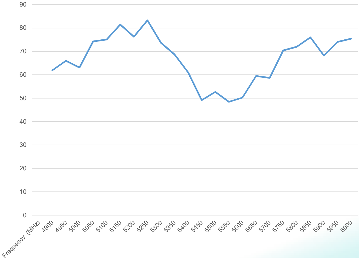
ICEFIN49DMN Efficiency (%)
