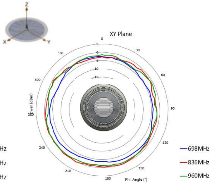
Horizontal Plane
