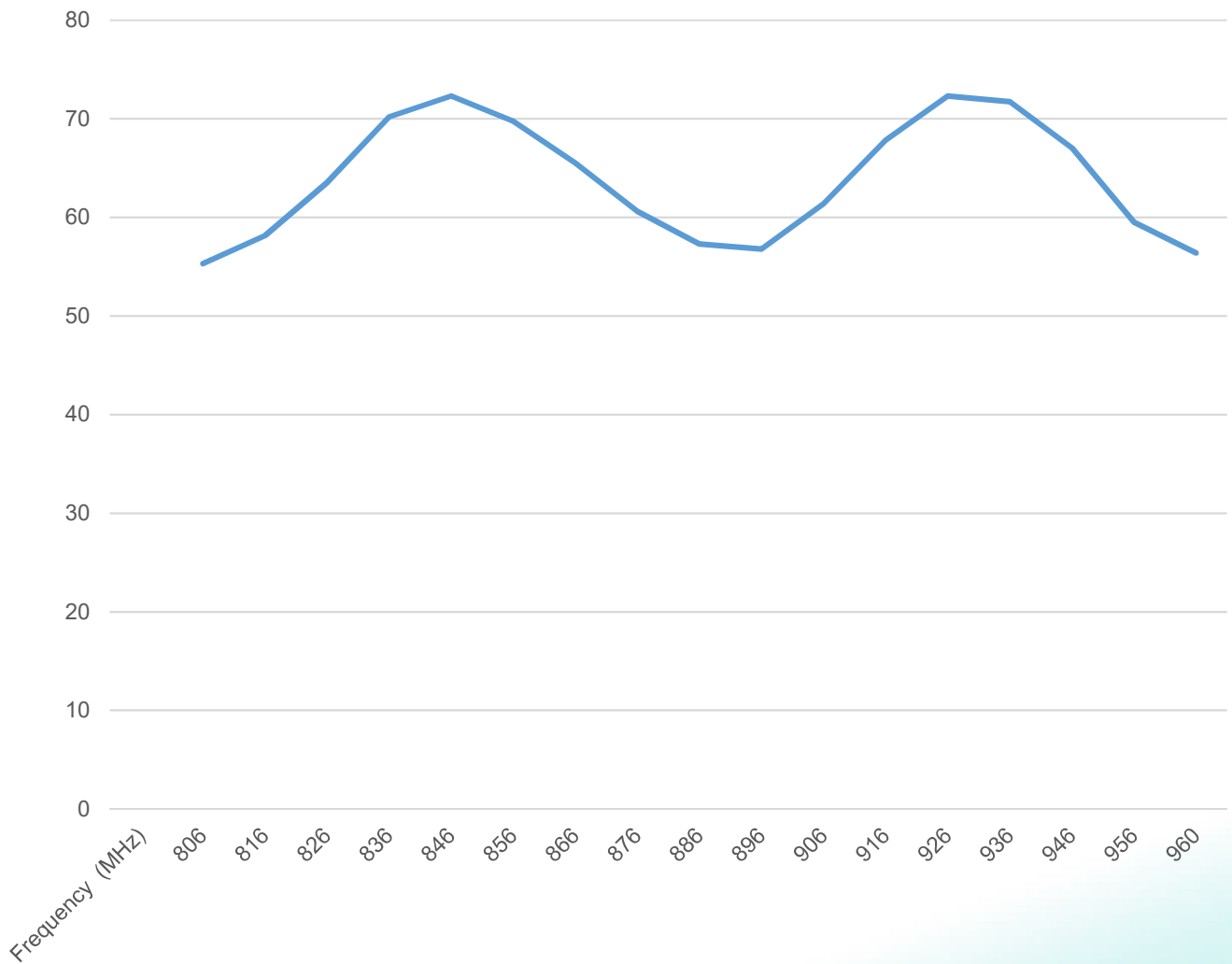
ICEFIN806NMO Efficiency (%)
