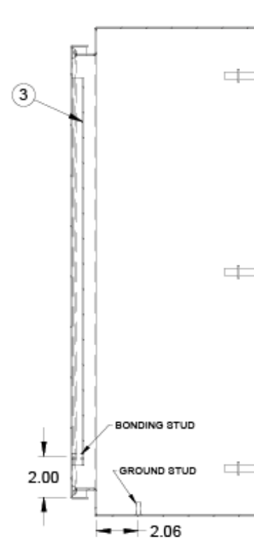
SECTION X-X
