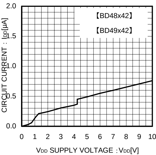
Fig.3 Circuit Current
