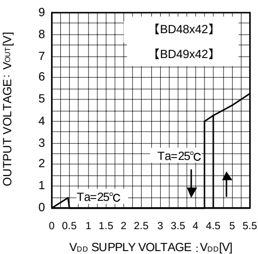
Fig.6 I/O Characteristics
