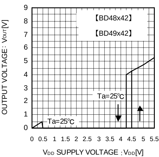
Fig.6 I/O Characteristics
