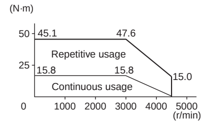
R88M-G4K030T (4 kW)
