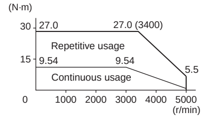
R88M-G3K030T (3 kW)
