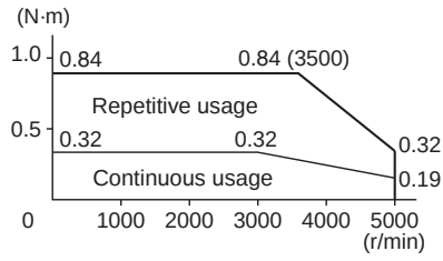
R88M-GP10030L/S (100 W)
