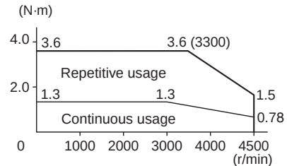
R88M-GP40030L/S (400 W)
