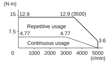
R88M-G1K530T (1.5 kW)
