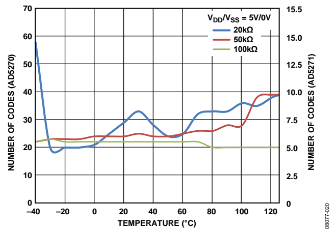
Figure 36. Maximum Code Loss vs. Temperature
