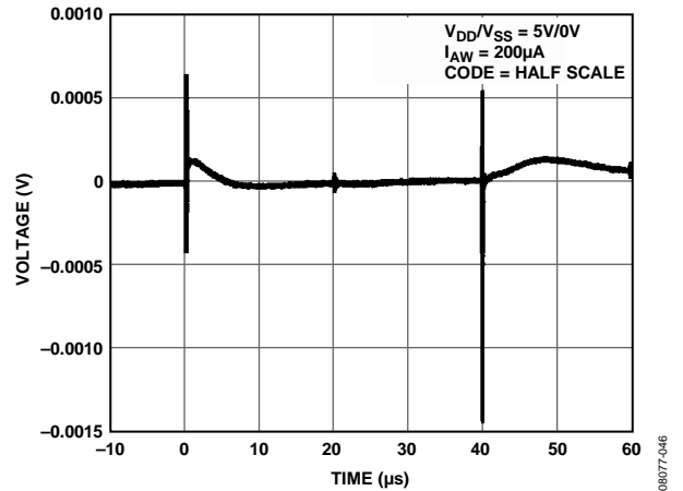
Figure 35. Digital Feedthrough
