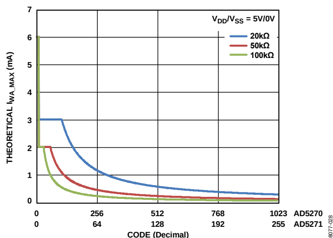
Figure 28. Theoretical Maximum Current vs. Code
