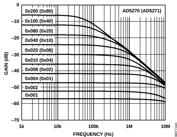
Figure 29. 100 kΩ Gain vs. Code vs. Frequency
