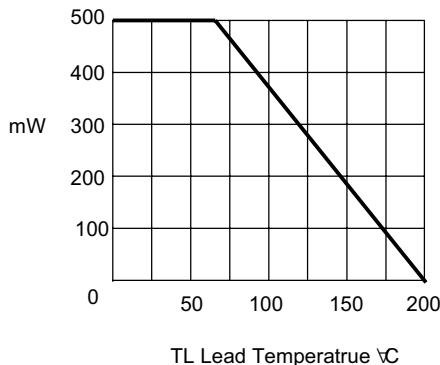
Figure 2 - Derating Curve
