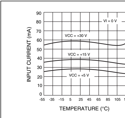
Figure 6. Input current
