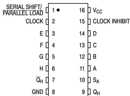
Figure 1. Pin Assignment
