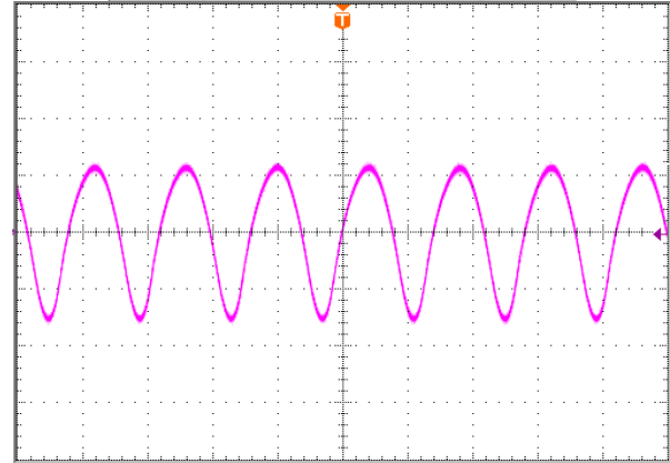
Figure 9: Input Terminal Ripple Current, i_c , at full rated output current and nominal input voltage ( V_{in}=48V ) with 12µH source impedance and 33µF electrolytic capacitor (250mA/div, 2µs/div)
