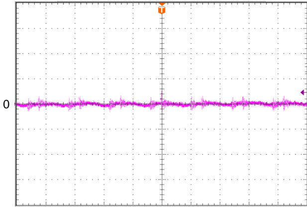
Figure 10: Input reflected ripple current, i_s , through a 12µH source inductor at nominal input voltage ( V_{in}=48V ) and rated load current (5mA/div, 2µs/div)
