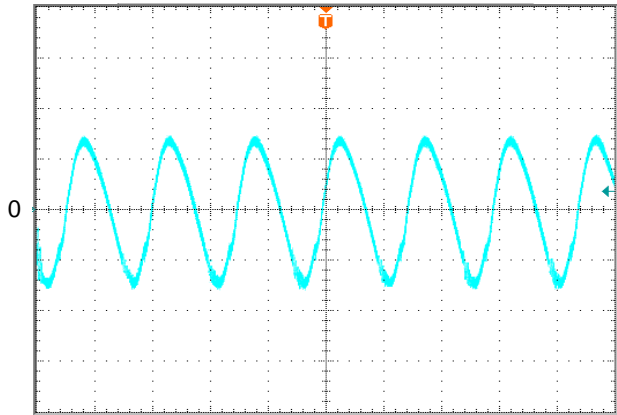
Figure 12: Output voltage ripple at nominal input voltage ( V_{in}=48V ) and rated load current ( I_o=9A ) (20mV/div, 2µs/div). Load capacitance: 1µF ceramic capacitor and 10µF tantalum capacitor. Bandwidth: 20 MHz. Scope measurements should be made using a BNC cable (length shorter than 20 inches). Position the load between 51 mm to 76 mm (2 inches to 3 inches) from the module
