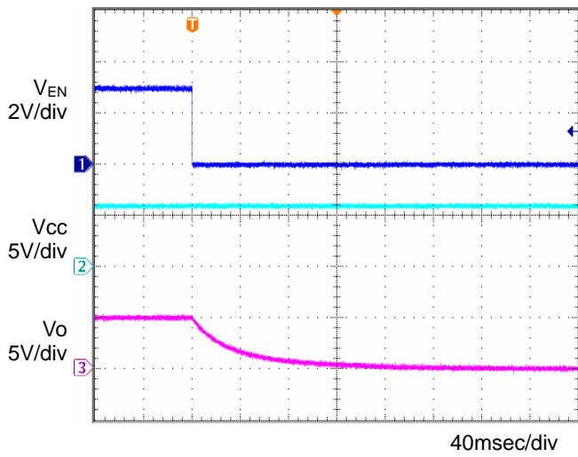
Fig.19 OFF sequence 2 Co=1 \mu F, Ta=25°C
