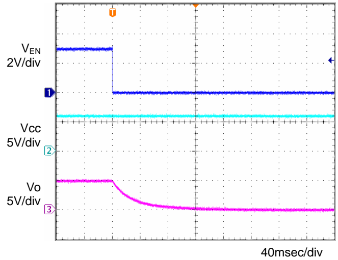
Fig.20 OFF sequence 2 Co=1 \mu F, Ta=105°C
