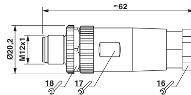
Dimensioned drawing
