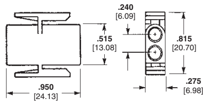
Socket Housing (Plug) Part No. 1-350344-0
